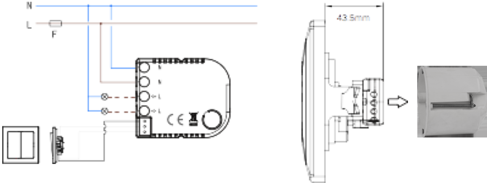
Wall mounting
